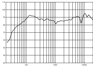
Frequency response on axis 1W/1m
