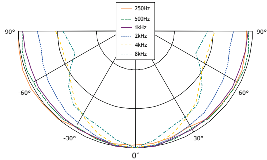
Directivity pattern
